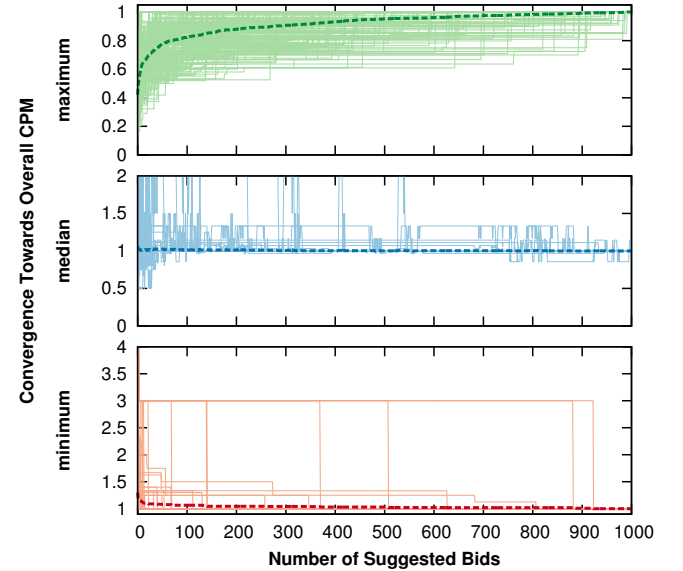
Figure 9: Convergence of different numbers of collated suggested bids towards overall CPM minimum, median, and maximum values for each of the 204 countries (each country is represented by a line in each graph). The average value across all countries is shown as the dark dashed line. Very quick convergence is observed for minimum and median, as expected.
