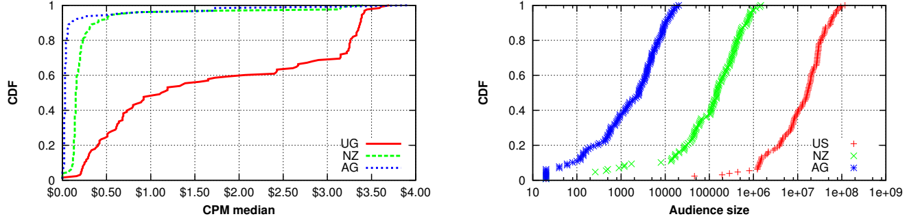
Figure 12: (a) Cumulative distribution of CPM median values for 129 interest categories for three countries. (b) Cumulative distribution of audience size for three countries (United States, New Zealand, and Antigua and Barbuda).
