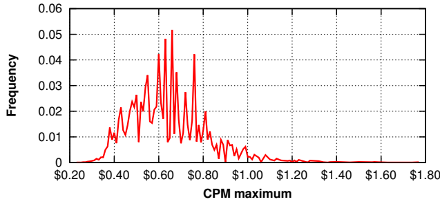
Figure 6: Example probability distribution function of CPM maximum values for 20,000 successive suggested bids (US 25-year-old females interested in computer programming; 179,760 users). This distribution fails statistical tests for multiple common distributions, suggesting the absence of random noise.
