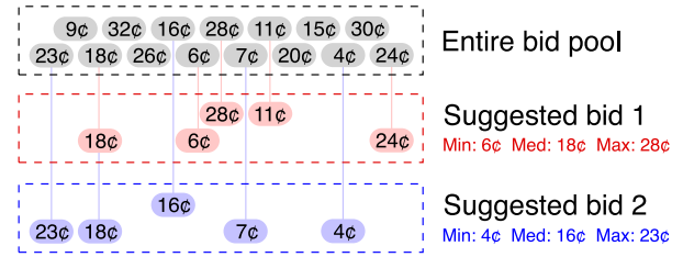
Figure 8: Diagram of Hypothesis 3: Sampling winning bids. To generate each suggested bid, Facebook selects a sample of bids from the set of all bids, and returns the median, minimum, and maximum from the sample.
