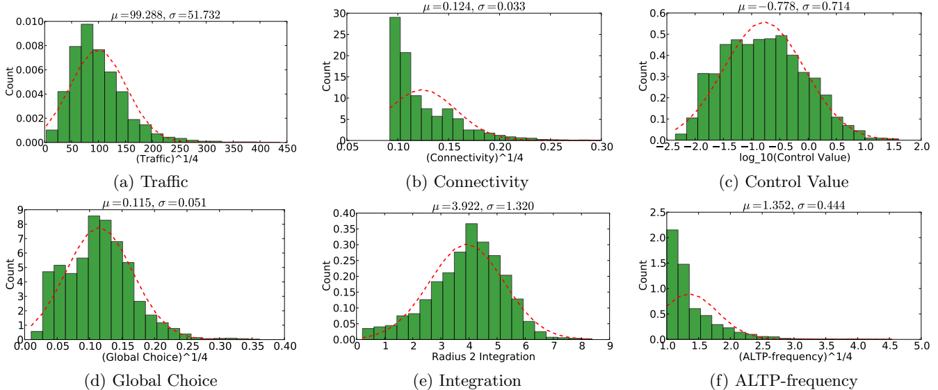
Figure 7: Distribution of the transformed different metrics and traffic volume for all AS-links discovered in the April 2011 traceroute datasets for IXP . Similar distributions are observed for the other datasets and the two studied network entities.
